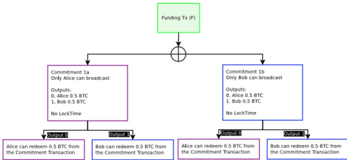
Figure 3: Purple boxes are unbroadcasted transactions which only Alice can broadcast. Blue boxes are unbroadcasted transaction which only Bob can broadcast. Alice can only broadcast Commitment 1a, Bob can only broadcast Commitment 1b. Only one Commitment Transaction can be spent from the Funding Transaction output. Blame is ascribed, but either one can still be spent with no penalty.
