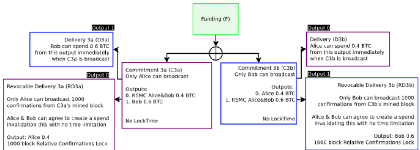
Figure 13: Since Bob proved to Alice he knows R by telling Alice R , Alice is willing to update the balance with a new Commitment Transaction. The payout will be the same whether C2 or C3 is broadcast at this time.
